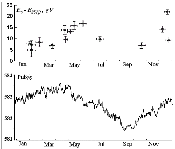
Fig. 5. Top: the Troitsk experiment. Difference between theoretical and experimental ranges of the \beta decay spectrum of tritium near maximum energy as a function of the time of year (1994-2001) [19]. Bottom: averaged count rate of a \beta source ^{90}\text{Sr} - ^{90}\text{Y} (2000-2007) [3].
