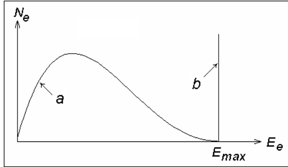
Fig. 2. Electron (positron) spectrums of normal (a) and reverse (b) \beta decays initiated by low energy neutrino. N_e - number of emitted electrons (positrons), E_e - energy of electrons (positrons), E_{max} - maximal energy of \beta spectrum.
