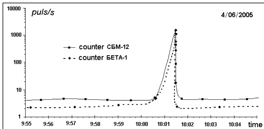
Fig. 4. An example of a burst of the count rate of a \beta source mounted at the focal point of a mirror with parabolic surface. Radiation from a ^{60}\text{Co} sample was registered by means of two independent Geiger counters [3, 17].
