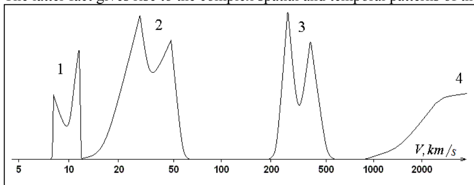
Fig. 1. Aspect of distribution of dark matter fluence versus velocities of meeting with a surface of the Earth [3]. 1 – near-Earth particles, 2 - Solar system particles, 3 - galactic, 4 - extragalactic particles.
